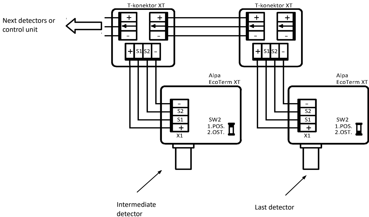
Figure 6: Settings of the configuration switch
