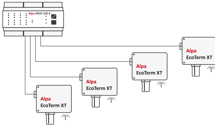
Figure 2: Connection with the Alpa MOD LED8 control unit into a star-shaped system
