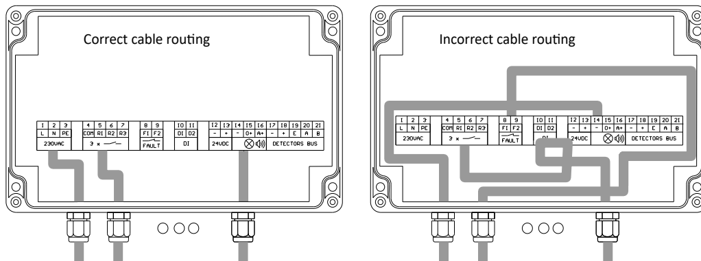
Figure 7: Example connection of cables to the device
