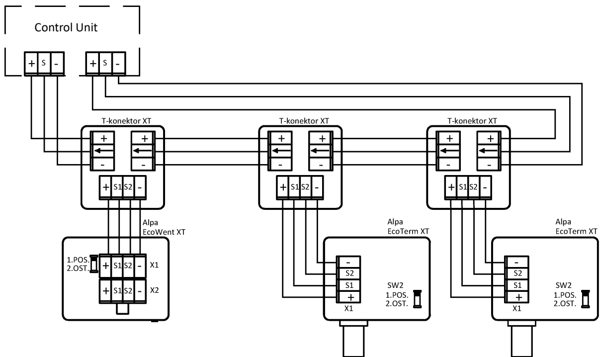
Figure 10: Closed alarm loop
