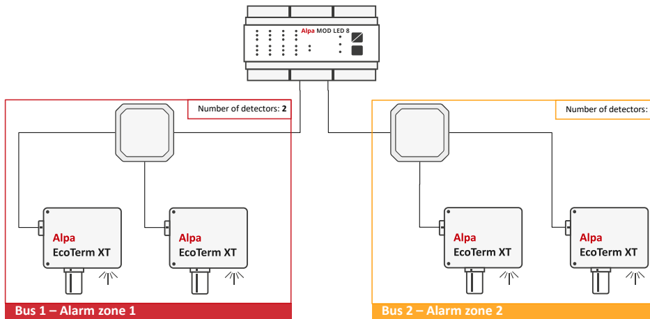
Figure 5: Connecting into two open bus systems servicing two zones
