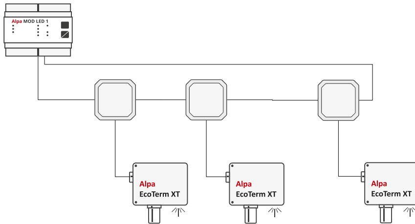
Figure 4: Connection with the Alpa MOD LED1 control unit into a closed bus system
