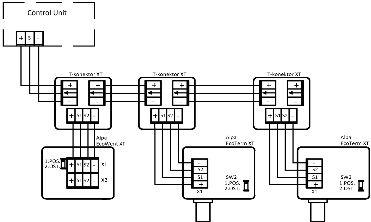
Figure 9: Open bus system
