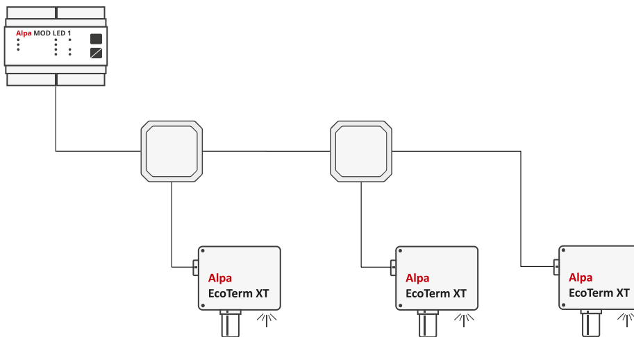
Figure 3: Connection with the Alpa MOD LED1 control unit into an open bus system
